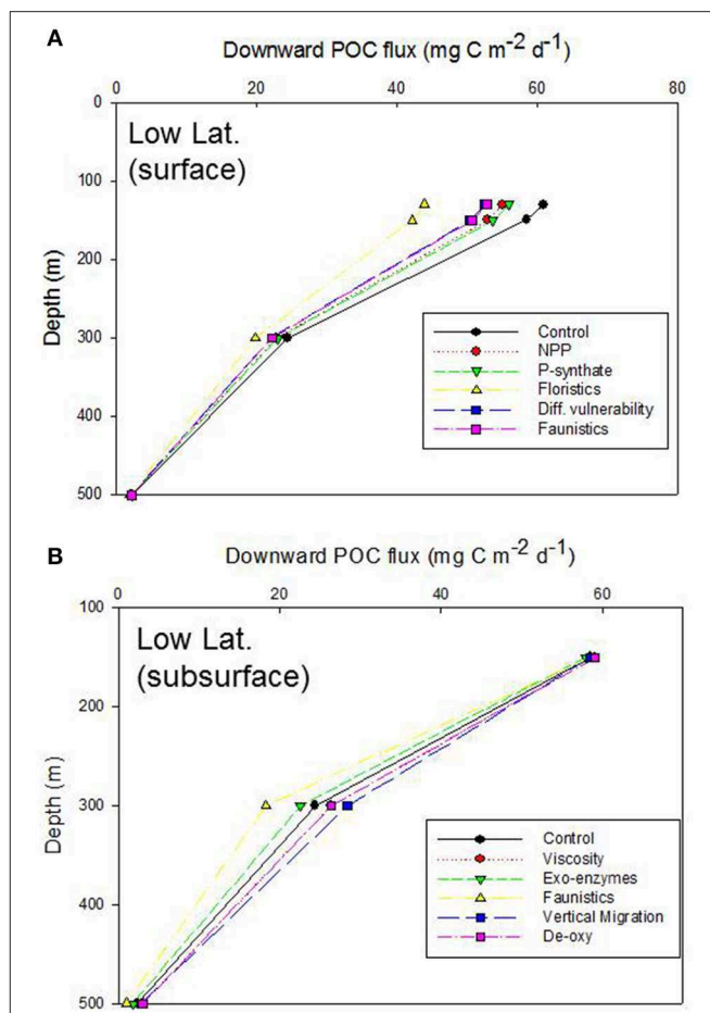
FIGURE 5 | Vertical profile of projected POC flux for the control run, low latitude case. The additional simulations for (A,B) are as described in Figures 4A,B . As for Figure 4B , the “Viscosity” profile is overlaid by “De-oxygenation.” In the case of the NPP run, NPP is decreased for low latitudes (Bopp et al., 2013; Marañón et al., 2014). Note, the convergence of fluxes at 150 m depth is due to relatively little influence of altered subsurface processes over 20 m depth (i.e., 130 m deep E_z , Table 2 ).
