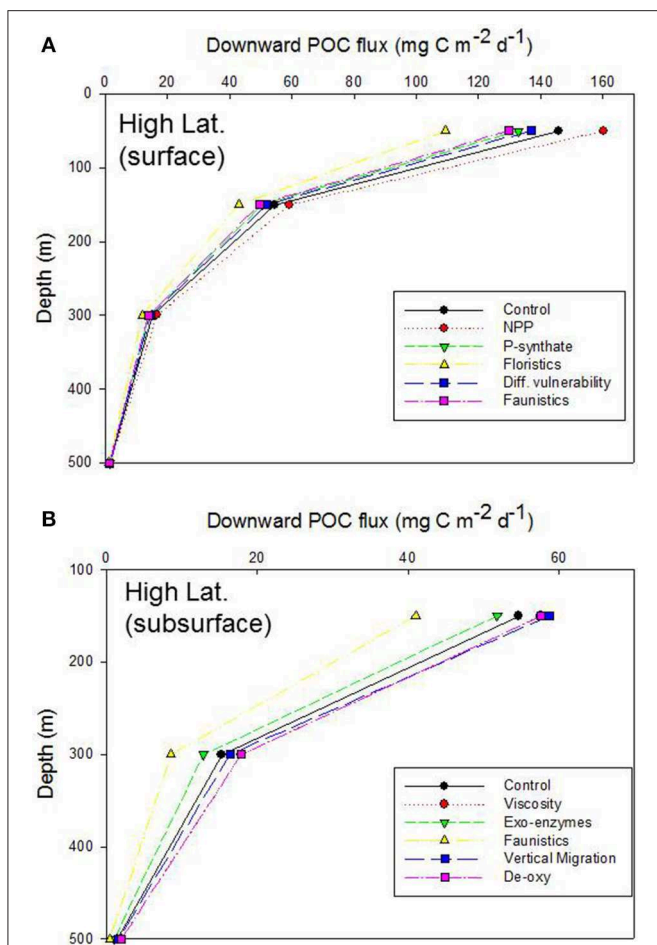
FIGURE 4 | Vertical profile of projected downward POC flux for the control run, high latitude case. Note that the profile for the Viscosity run is overlaid by that for De-oxygenation. (A) Additional simulations represent the systematic alteration of the individual components of the pump for the surface ocean: NPP, increased NPP; P-synthate, NPP directed to bacteria resulting in increased BP; Floristics, altered size-partitioning of NPP; Diff. vulnerability, altered microzooplankton trophic transfer efficiency; Faunistics, altered mesozooplankton trophic transfer efficiency. (B) As for (A) , but the simulations represent the systematic alteration of the pump components for subsurface waters: Viscosity, decreased seawater viscosity increasing particle sinking rates; Exo-enzymes, more microbial activity; Faunistics, altered mesozooplankton trophic transfer efficiency; Vertical migration, altered vertical POC shunt; De-oxy, decreased microbial remineralization due to de-oxygenation.
