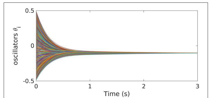
FIGURE 14 | Evolution of the controlled dynamics of the Kuramoto model (5) with N = 1,000 oscillators. The control has been computed with the GD-RBM algorithm.
